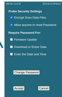
Security Settings
